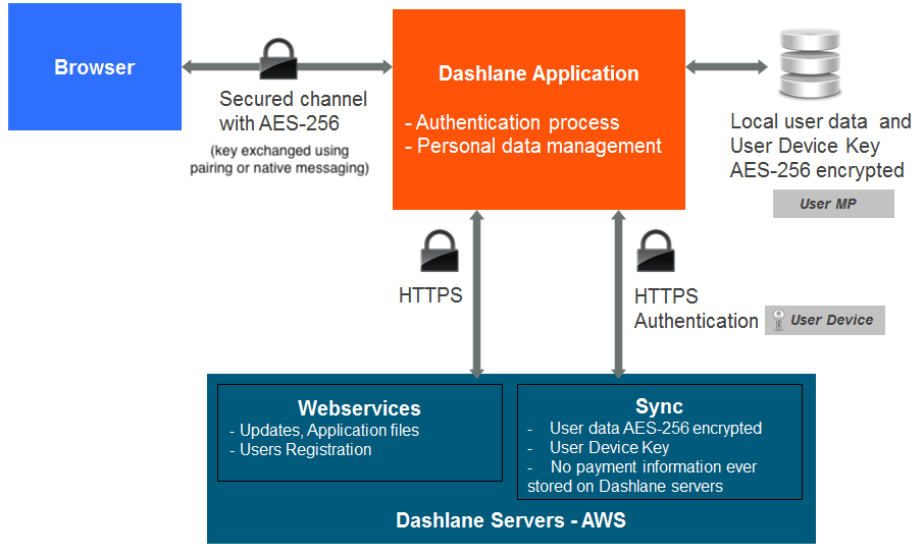
Figure 1: Use of Authentication Mechanisms in Dashlane
