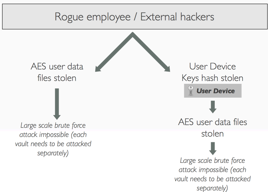
Figure 4: Limits on Attack Potential With Dashlane's Security Architecture
