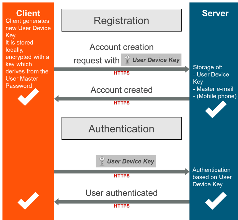
Figure 2: Authentication Flow During Registration
